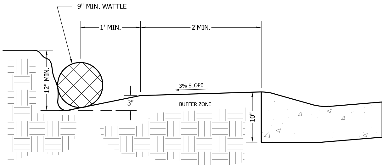
ROLLOVER CURB TYPE "B"
