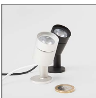
C1-S in display cases, 360° rotatable, 180° swivelling, with screw base or magnetic base
