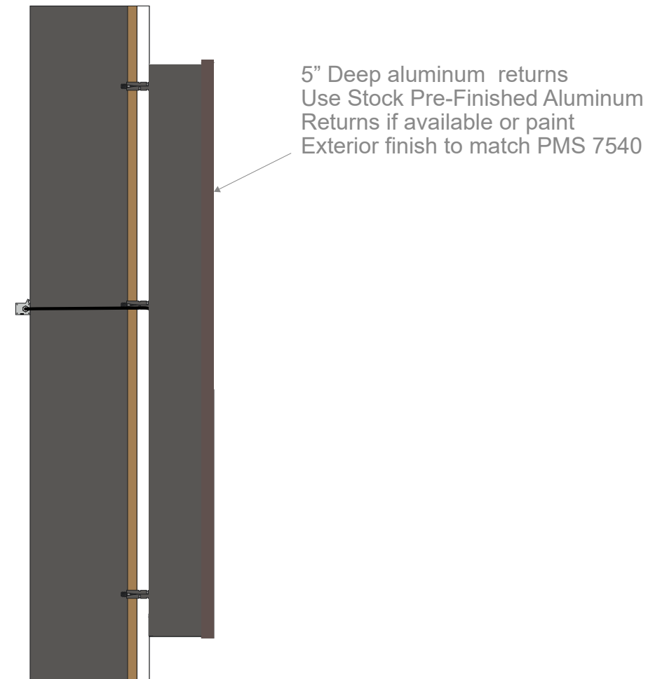
SIDE VIEW LETTERS DETAIL TYPICAL - N.T.S.
