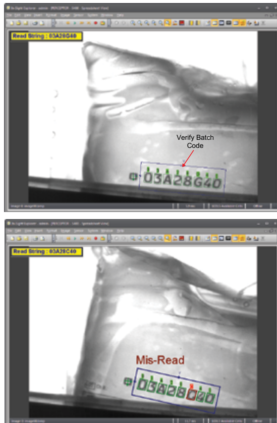
Figure 5. Machine-vision inspection using optical character recognition (OCR) to verify batch codes on soft plastic IV bags. This traceability application lets manufacturers track parts and products through the production facility and the supply chain.
