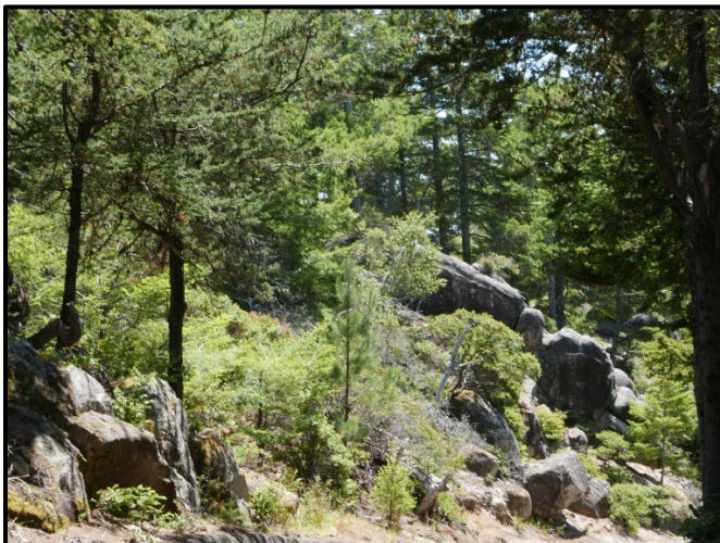
Figure H-7: A stand of Hesperocyparis pygmaea – Pinus muricata / Arctostaphylos nummularia Association over massive sandstone of the Seaside-Rock outcrop complex. Due to the large rocks, shrubs of A. nummularia and A. columbiana , are widely scattered. Fish Rock Road south of the Navarro River.
