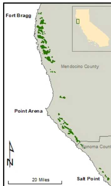
FIGURE 1. The Mendocino Cypress Woodland study area in Mendocino and Sonoma Counties is depicted in green.
