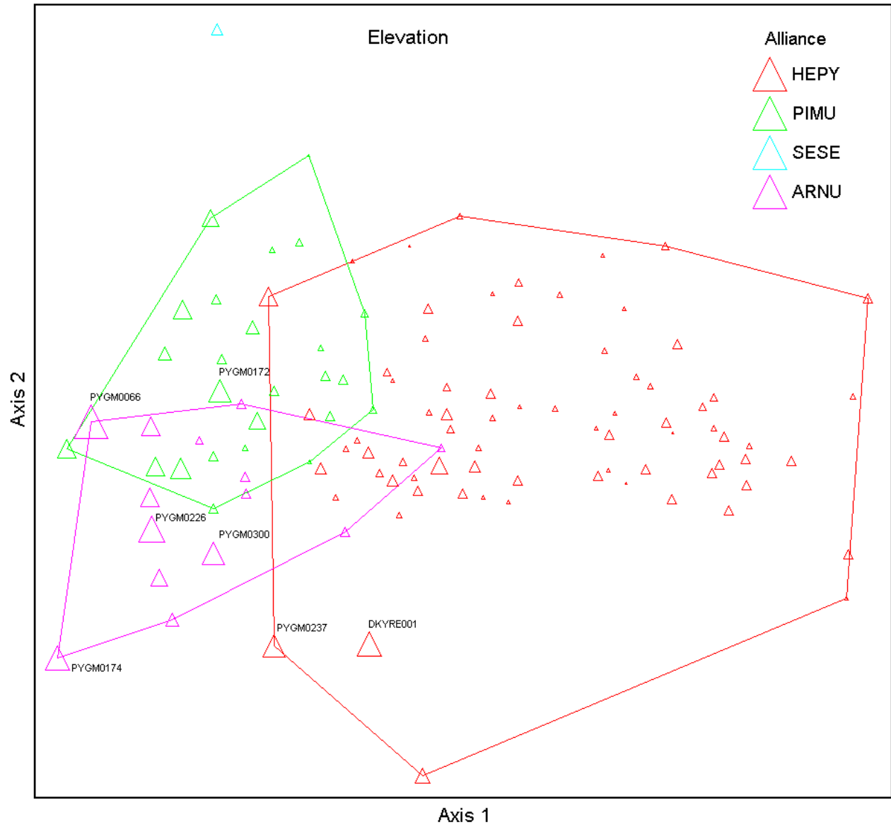
FIGURE 9. Samples plotted against Elevation. This diagram shows the relative elevation of samples assigned to the Hesperocyparis pygmaea (HEPY), Pinus muricata (PIMU), Sequoia sempervirens (SESE), and Arctostaphylos (nummularia, sensitiva) (ARNU) Alliances; relative elevation is indicated by the size of the sample triangles. Note that the seven samples with the highest elevations are associated with the lower left quadrant. Elevation is not positively associated with the distribution of mesic or wetland vegetation types.
