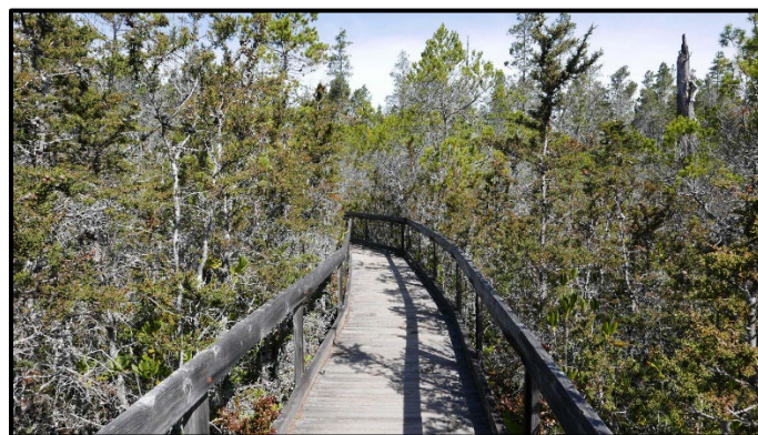
Figure H-6: A stand of Hesperocyparis pygmaea – Pinus contorta ssp. bolanderi – Pinus muricata / Rhododendron macrophyllum Association dominated by H. pygmaea averaging about 3m tall and 2.5cm diameter. Van Damme State Park pygmy forest boardwalk.
