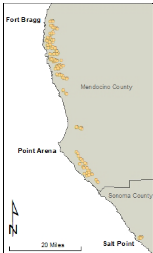
FIGURE 6. Locations of accuracy assessment samples collected in the Mendocino Cypress Woodland project.
