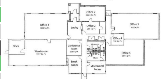
Building Plan View 1351 Aucutt Rd. Montgomery, IL.
