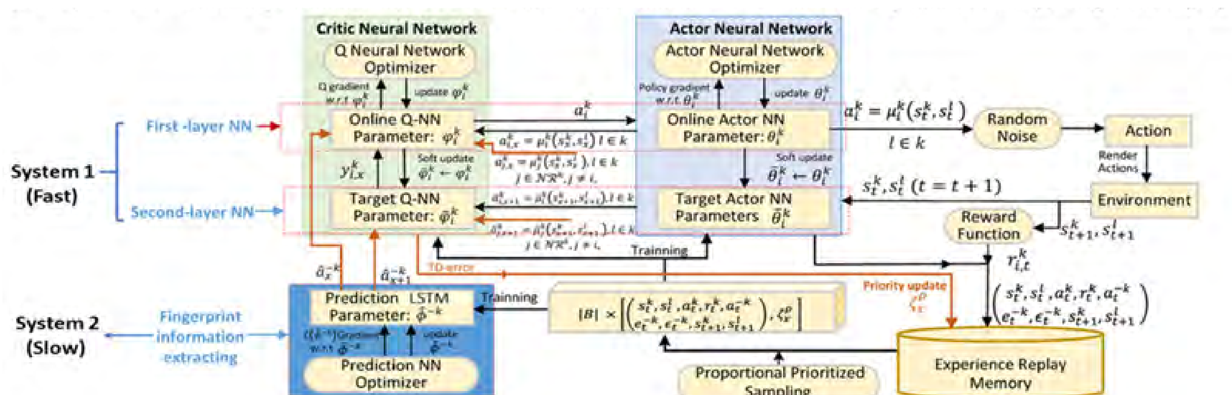
Fig. 3. Novel model architecture of a Long Short-Term Memory (LSTM)-based Fingerprint Networked Reinforcement Learning (FNRL) that shows multi-agent interaction based on multi-modal nonlinear and nonstationary data streams (Chang et al. in prep).
