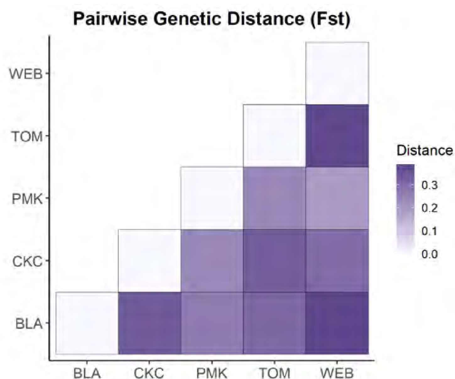
Figure 2. Pairwise genetic differentiation ( F_{st} ) among natural populations of Spartina based on multilocus genotypes.
