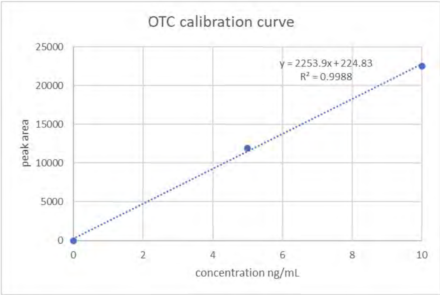
Figure 1. Standard curve for OTC calibration.
