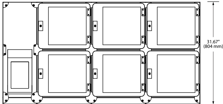
FRONT VIEW CUSTOMER SIDE
