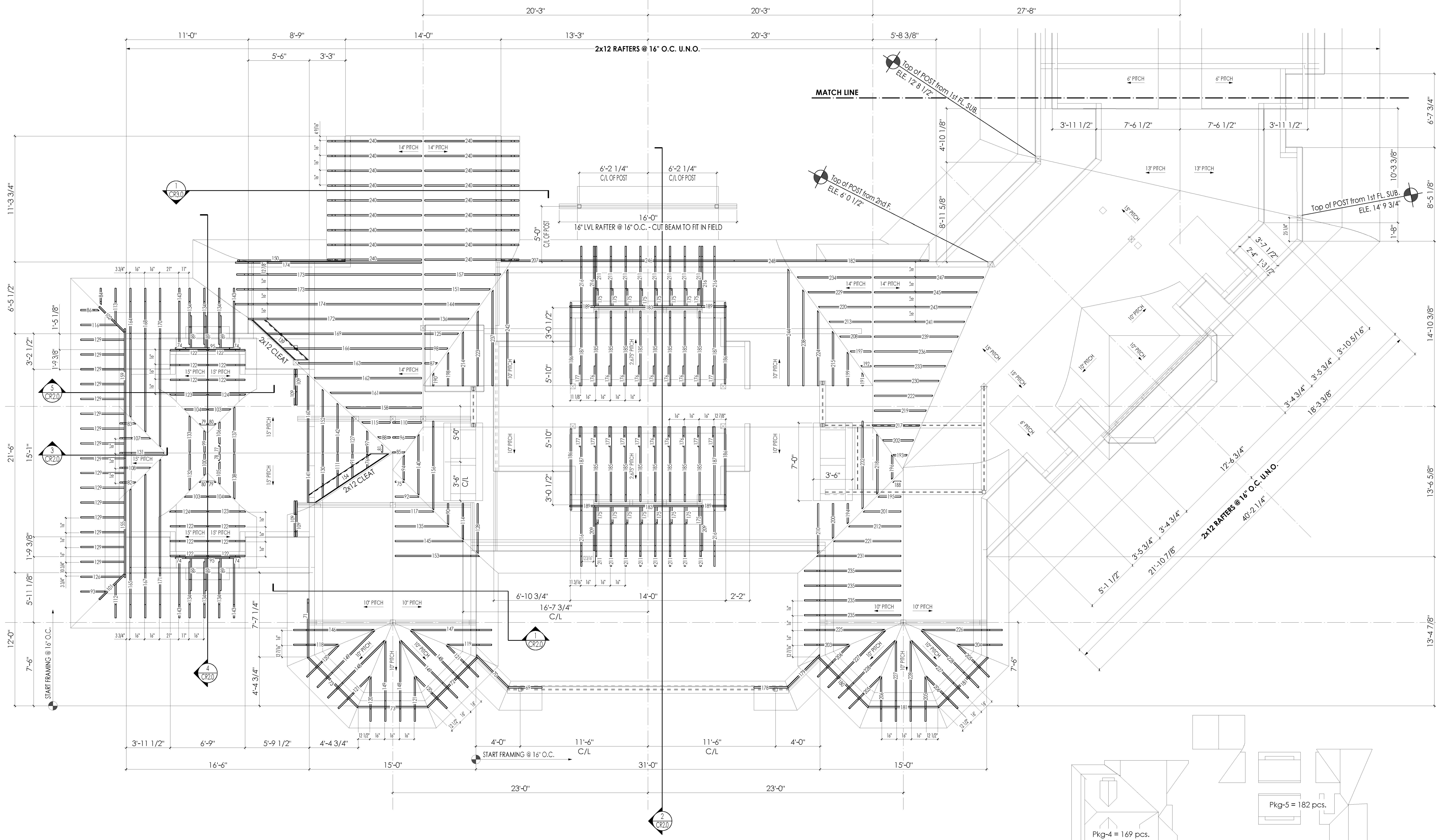
Pkg#4 & 5 ROOF FRAMING PLACEMENT PLAN SCALE: 1/4" = 1'-0"
