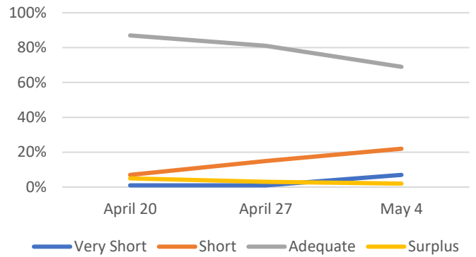
Topsoil Moisture
