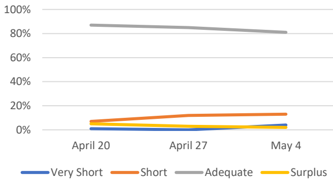
Subsoil Moisture
