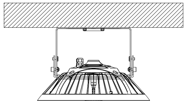
U-Bracket Mount
