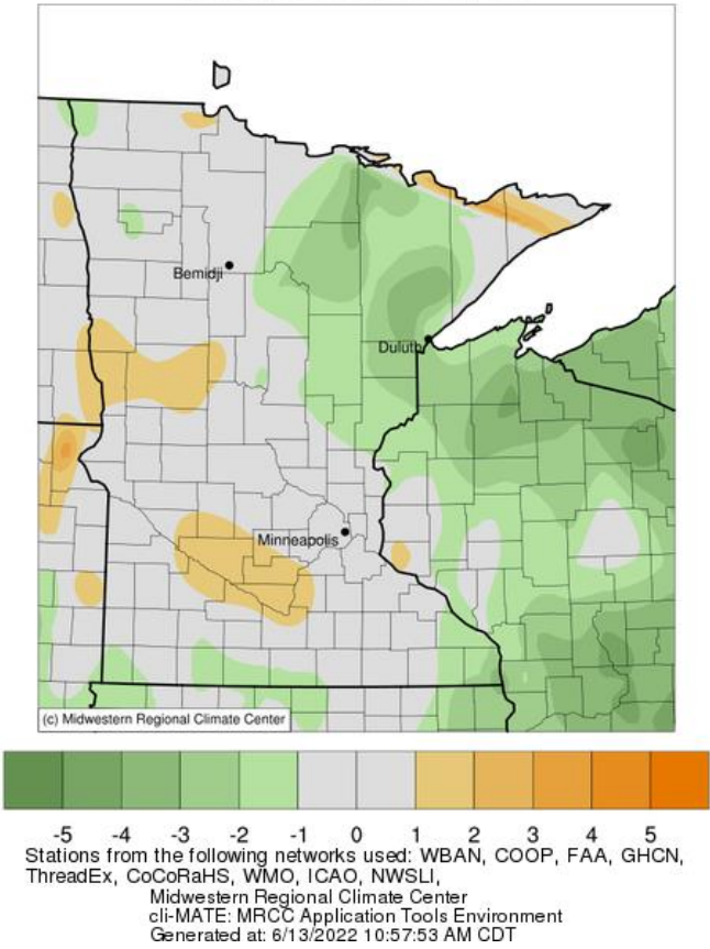
Average Temperature (°F): Departure from 1991-2020 Normals June 06, 2022 to June 12, 2022
