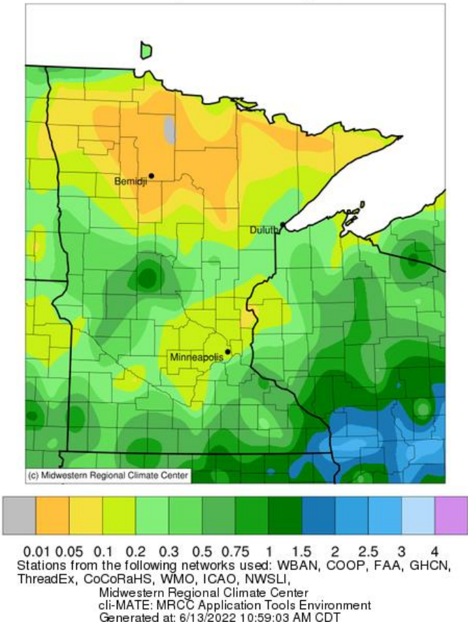
Accumulated Precipitation (in) June 06, 2022 to June 12, 2022
