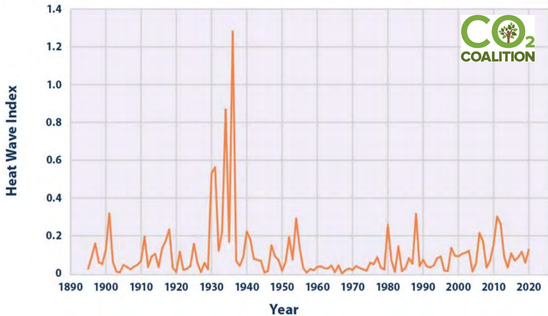
Figure 3. U.S. Annual Heat Wave Index, 1895–2020
