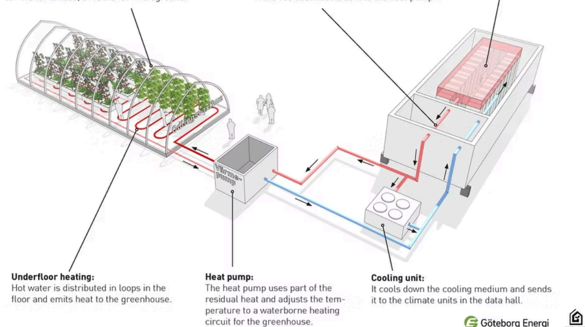
FIGURE 11. RENDERING OF INTERMEDIARY HEAT PUMP SUBSTATION BETWEEN GREENHOUSE AND DATA CENTER
