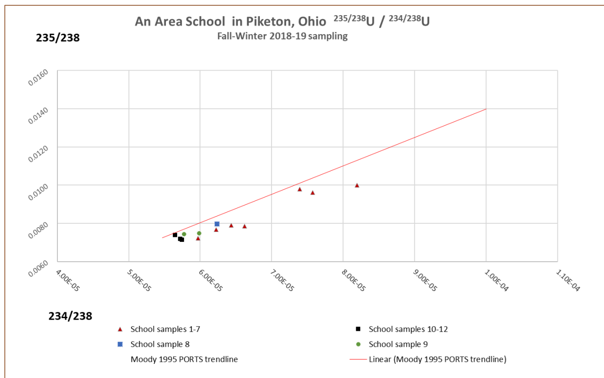
Figure 2. ^{234}\text{U} - ^{235}\text{U} - ^{238}\text{U} mixing diagram mixing diagram of samples collected at a Piketon-vicinity school in Fall/Winter 2018-2019. The mixing line of PORTS sample data from Moody (1995) is included for comparison.
