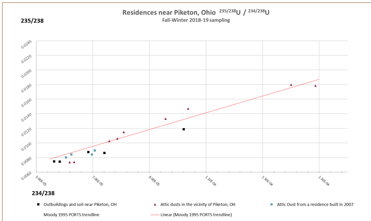
Figure 5. ^{234}\text{U} - ^{235}\text{U} - ^{238}\text{U} mixing diagram of soil and dust samples collected from residences near Piketon in Fall/Winter 2018-2019. The mixing line of PORTS sample data from Moody (1995) is included for comparison.
