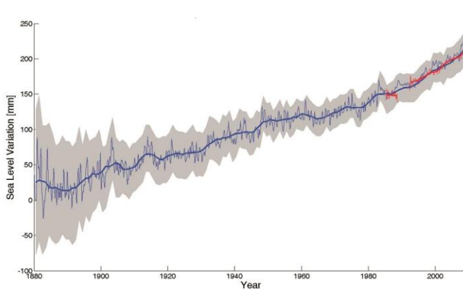
Chart 3: Sea level variation
