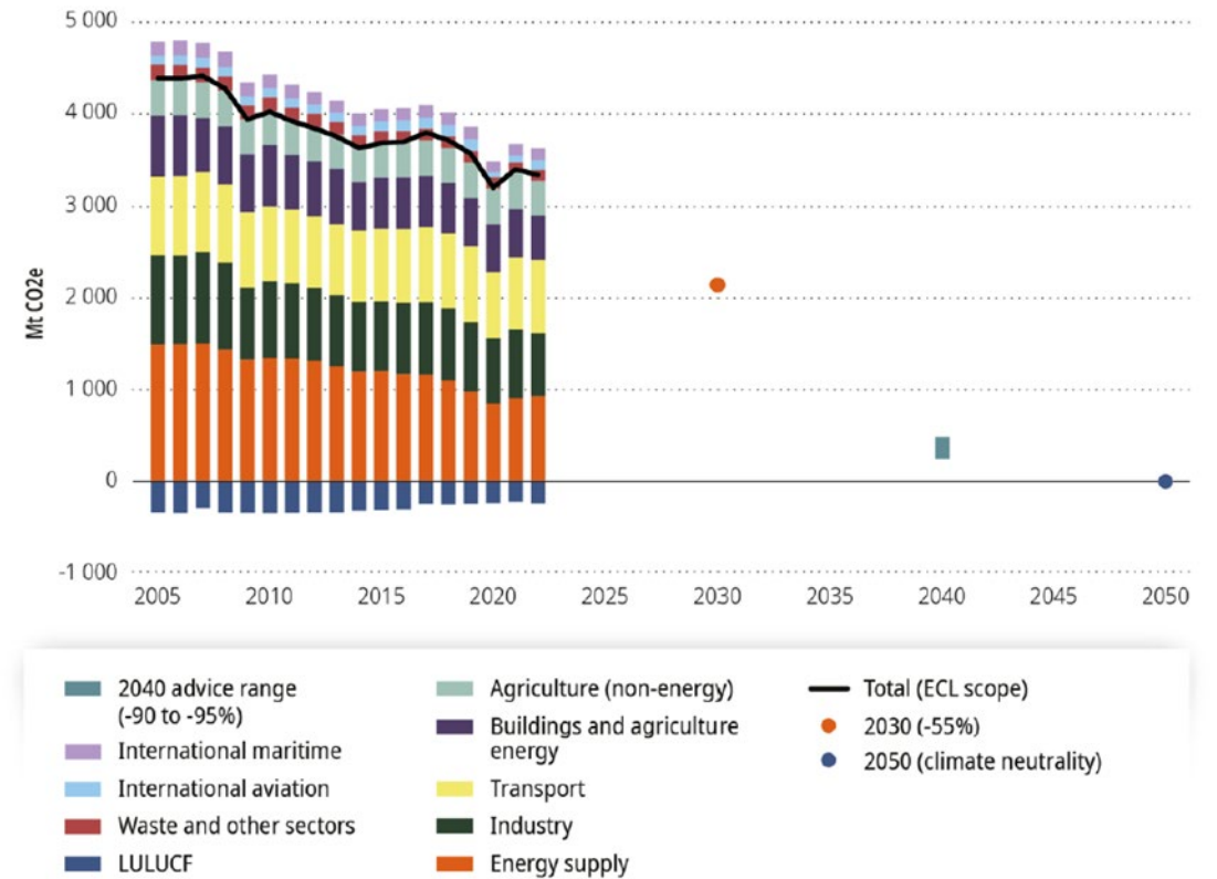
Figure 7 Indicator O1 – overall progress towards the EU's 2030 and 2050 GHG emission reduction objectives
