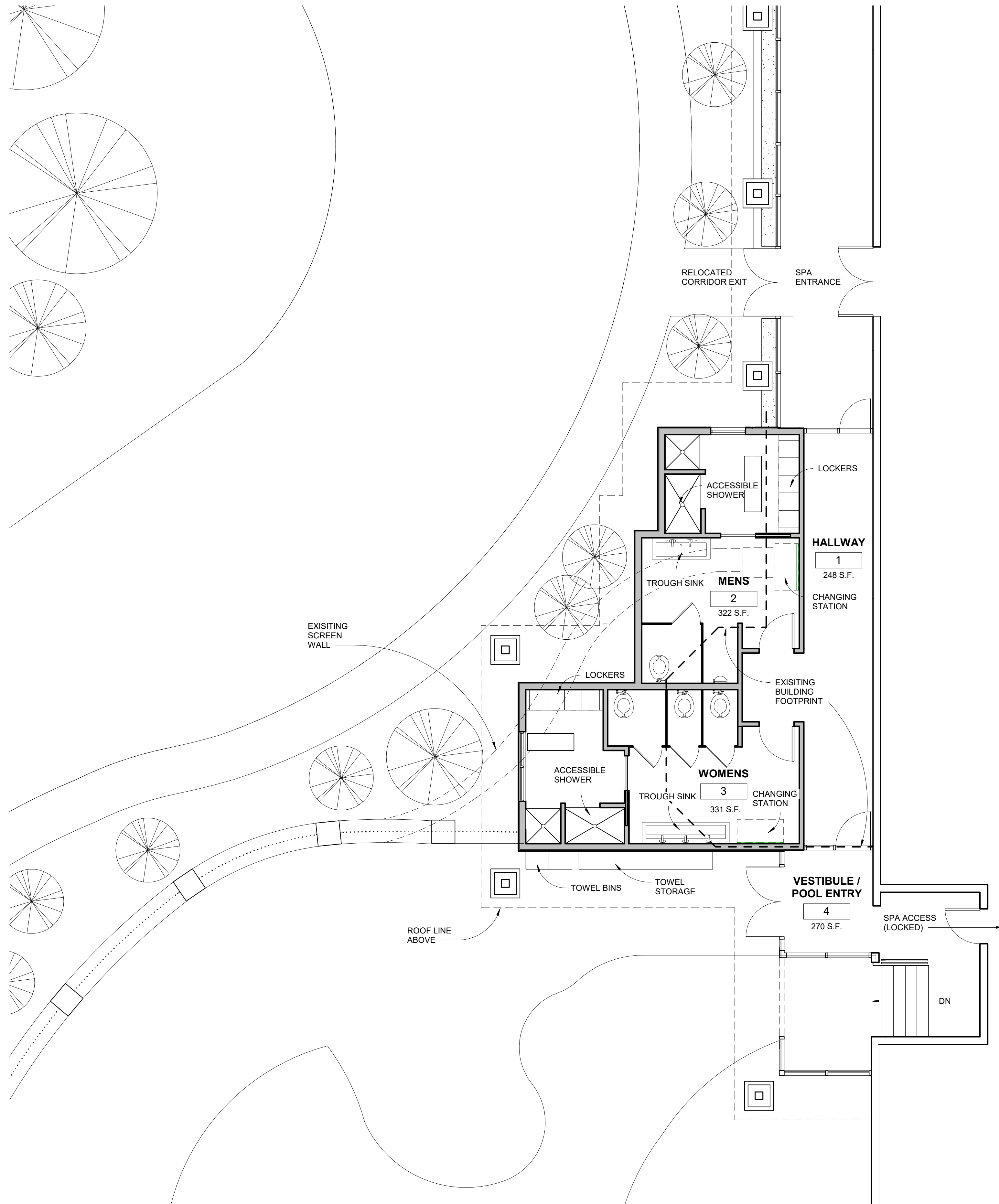
1 GROUND FLOOR LEVEL - SPA ENTRY 3/16" = 1'-0"
