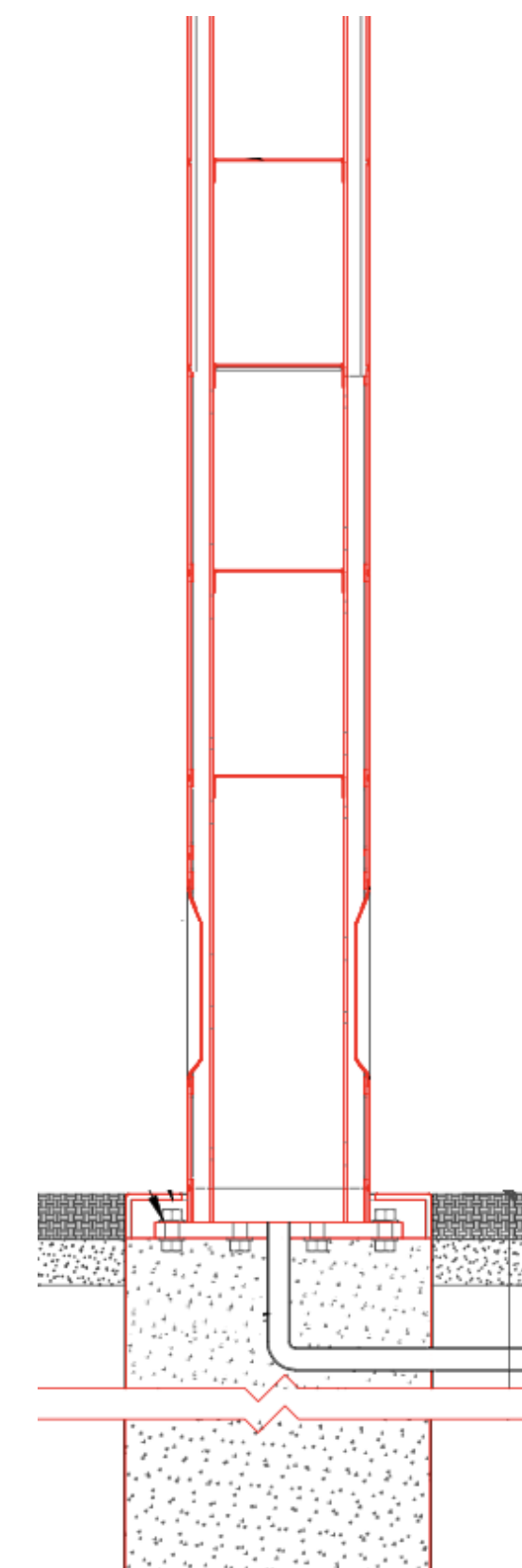
FOUNDATION SCHEMATIC
