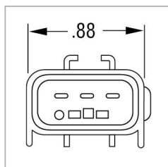
(3) Male Pins
