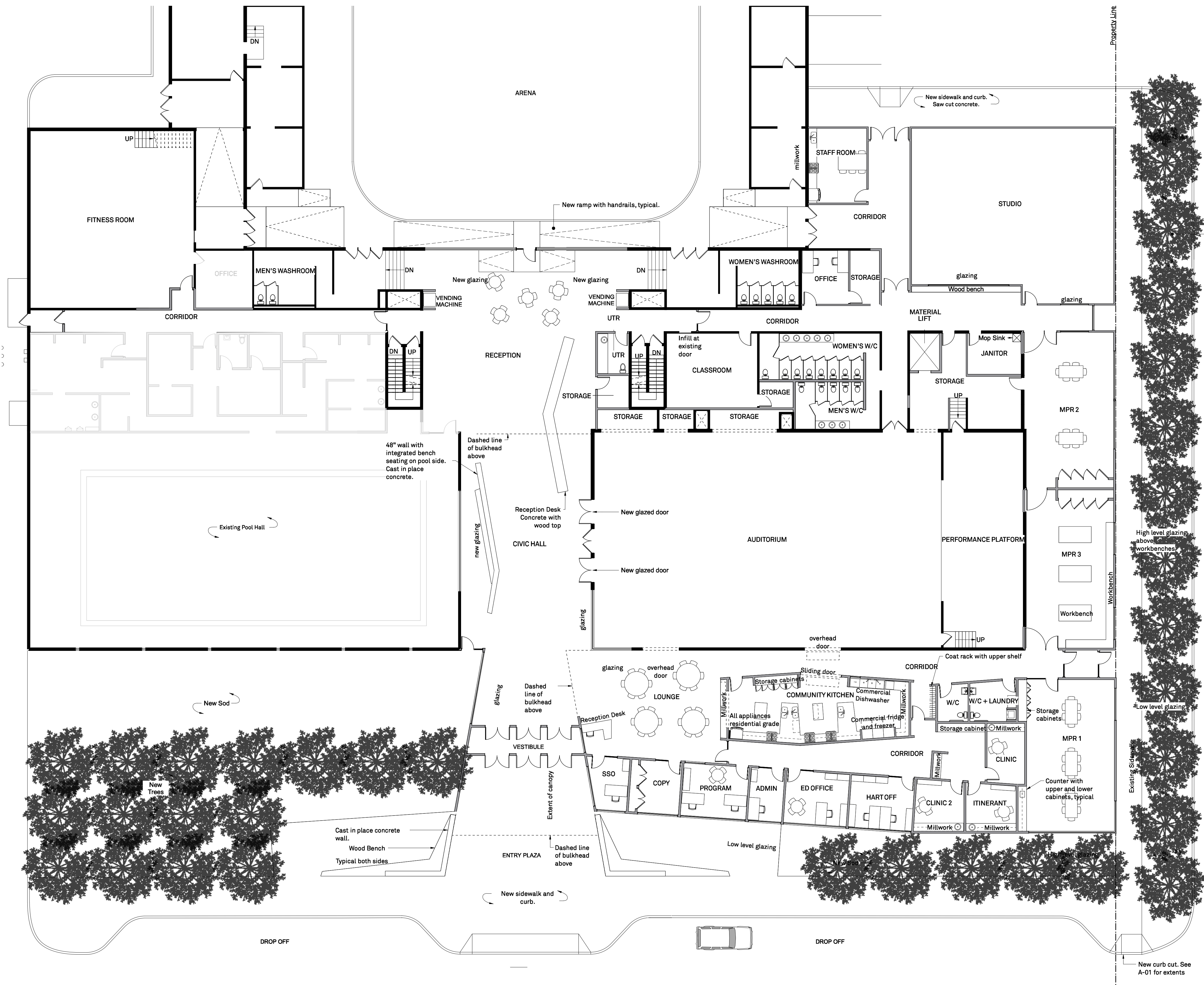
2 Renovation Plan - New Additions 1:150
