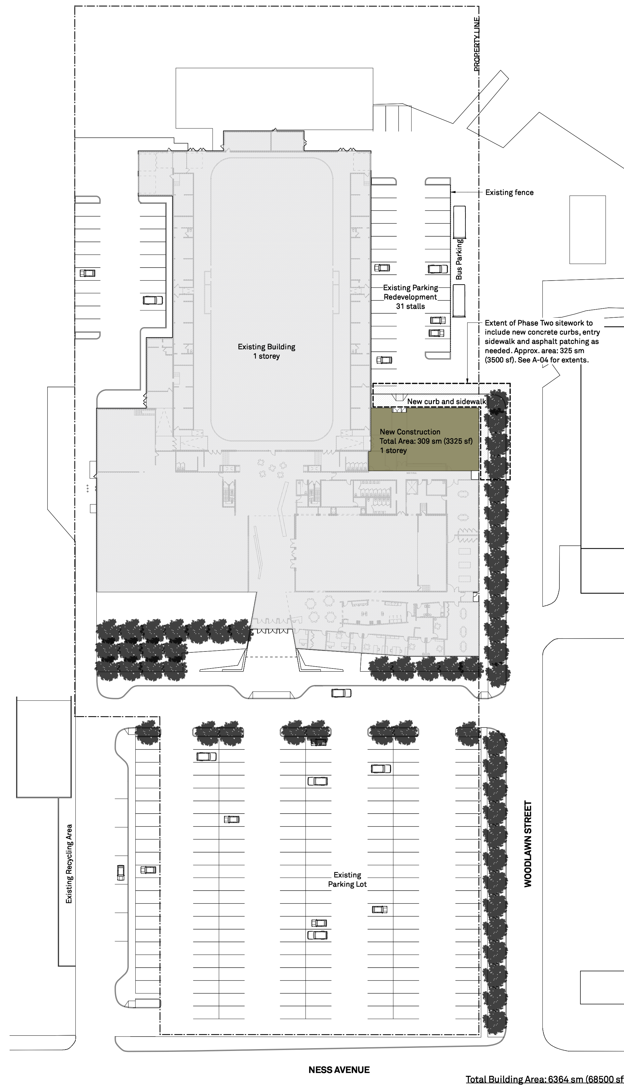
2 Site Plan - Part Two 1:500
