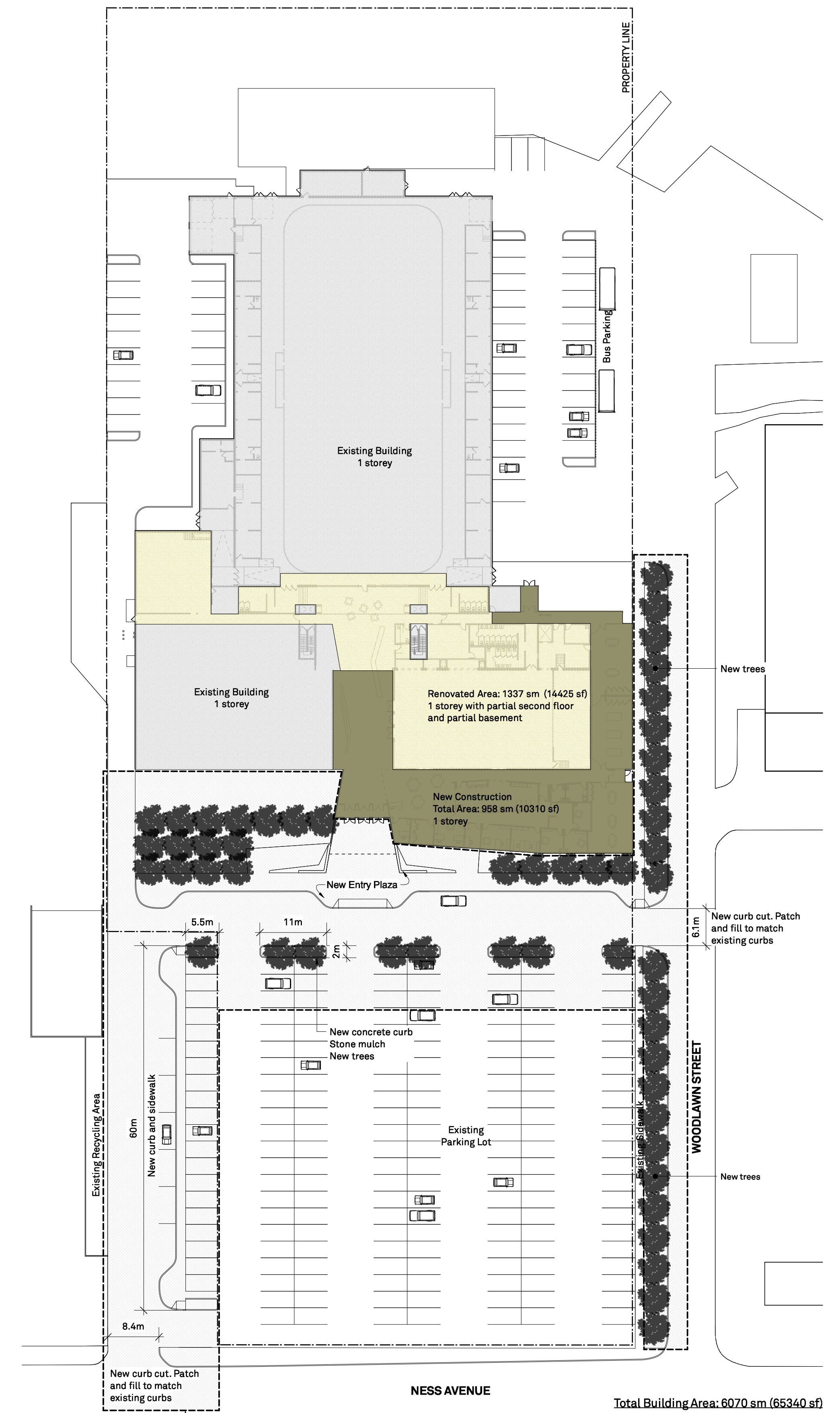
1 Site Plan - Part One 1:500
