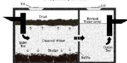
A Typical Septic Tank
