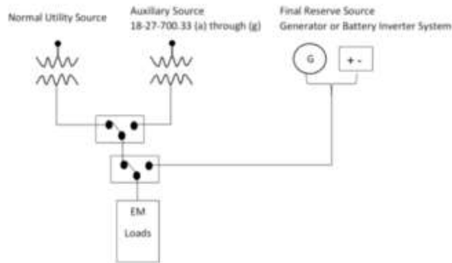
Figure 700.20 Typical System I Emergency System
