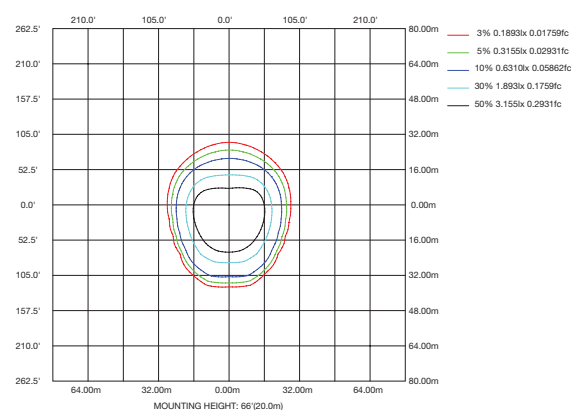
ISOLUX DIAGRAM
