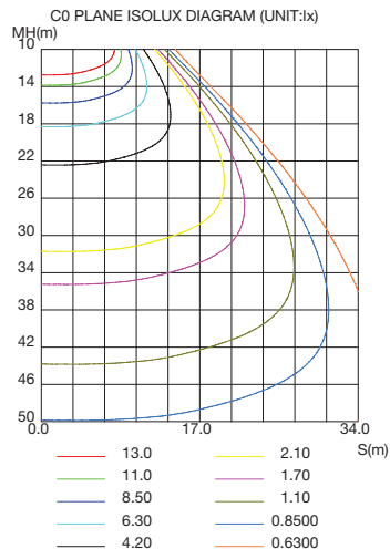
ISOLUX DIAGRAM
