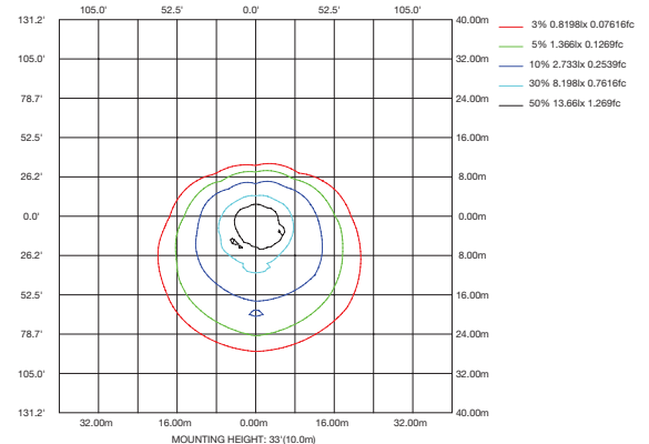
ISOLUX DIAGRAM
