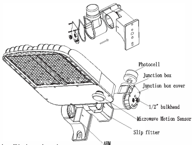
400W Shoebox Light Wiring drawing
