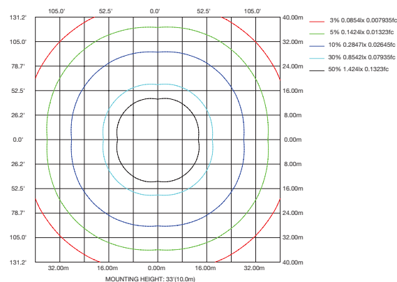
ISOLUX DIAGRAM
