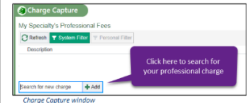
Charge Capture window
