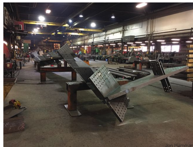
▲ A complex rib plate assembly in the shop.
