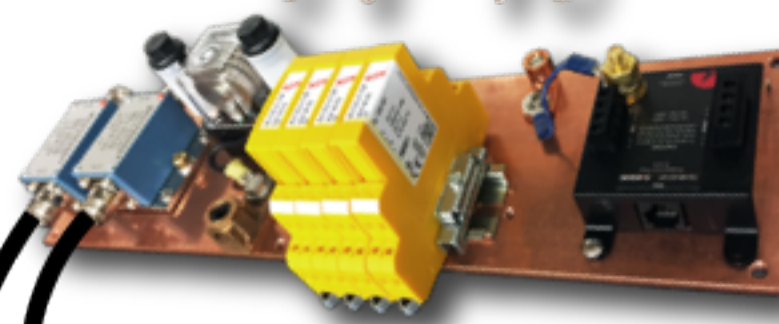
Surge Suppression Panel
