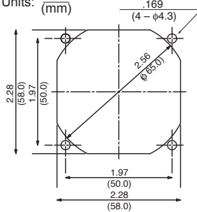
INLET SIDE
