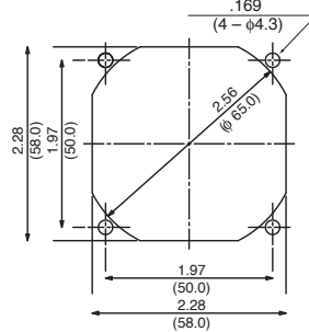
OUTLET SIDE
