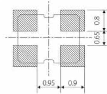
Figure 2) Land Pattern
