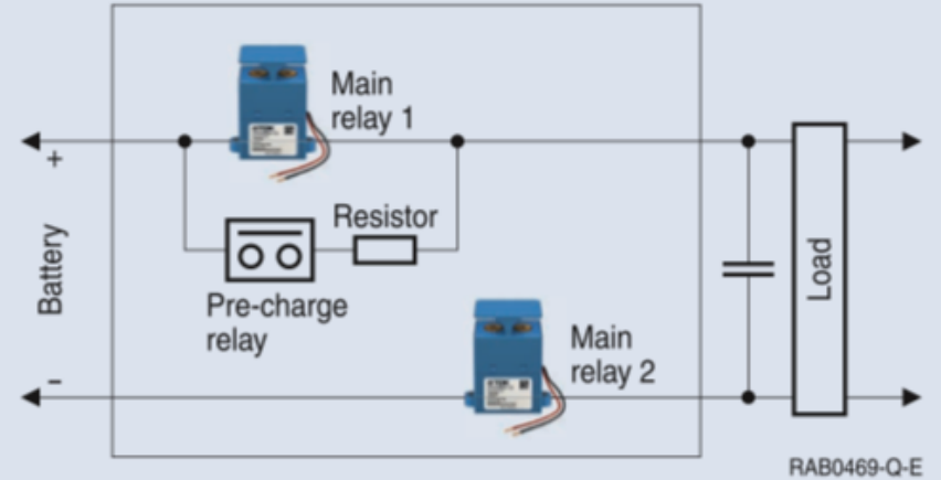
Battery disconnect unit
