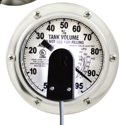
0023S00033 Module Cover on 5ANTS03047 Silver/Black Dial
