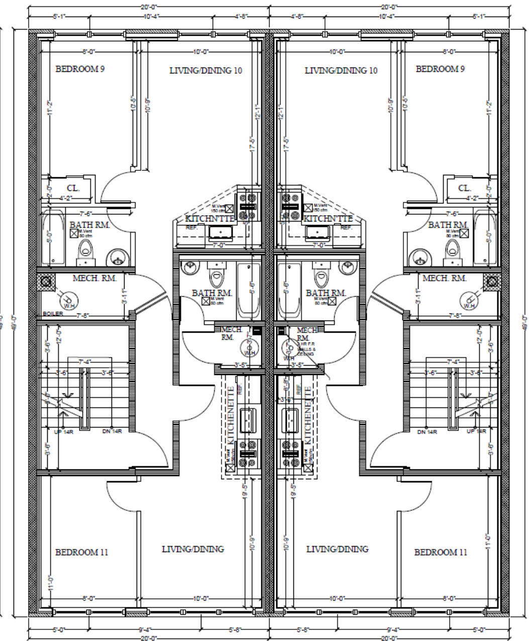
FOURTH FLOOR PLAN SCALE: 1/4"=1'-0"
