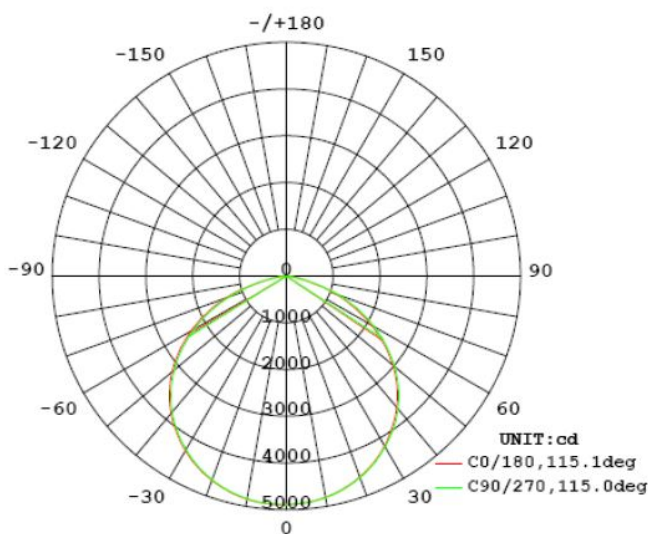
Luminous Intensity Distribution
