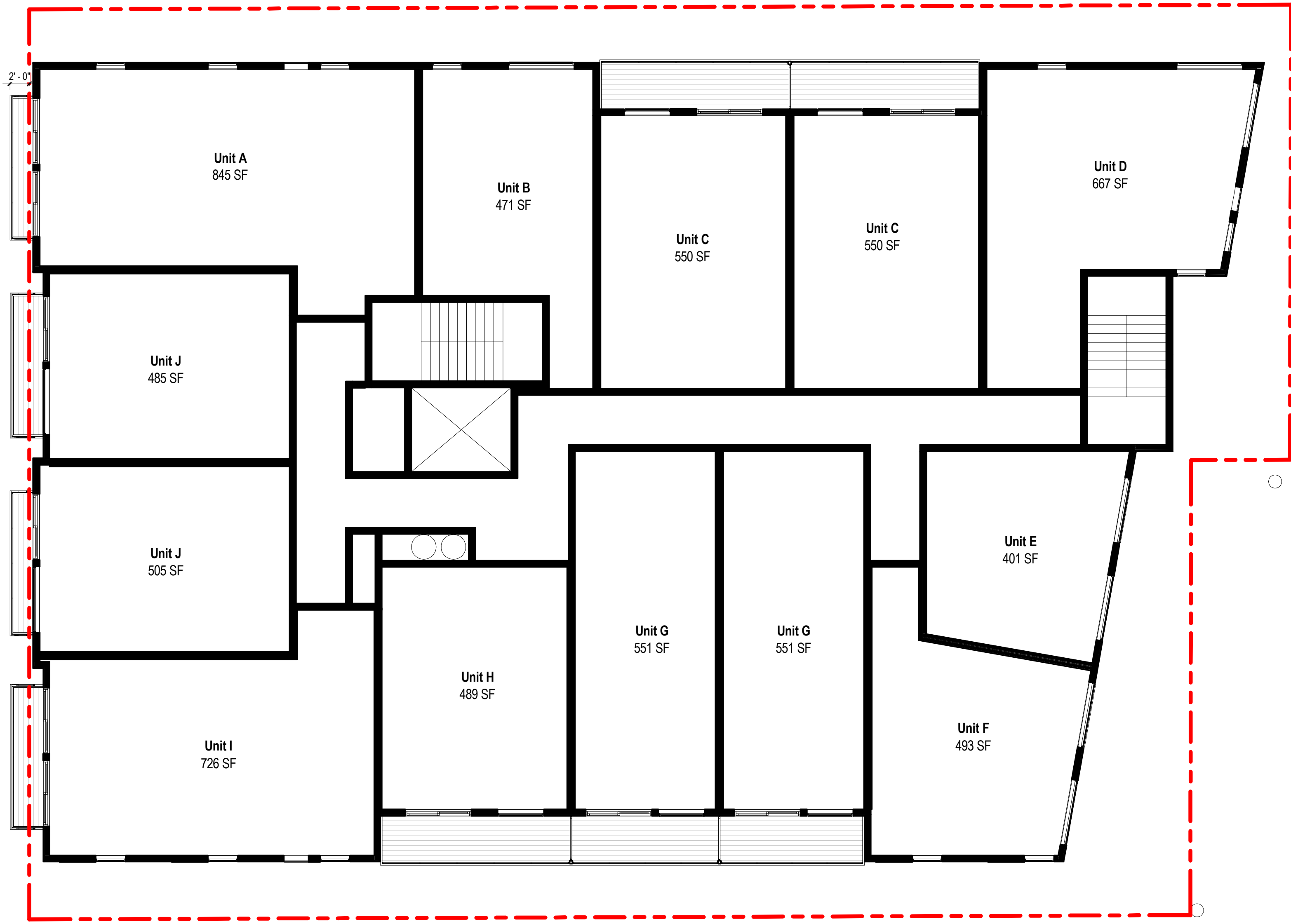
Plan - Typical Floor (3rd - 6th)
