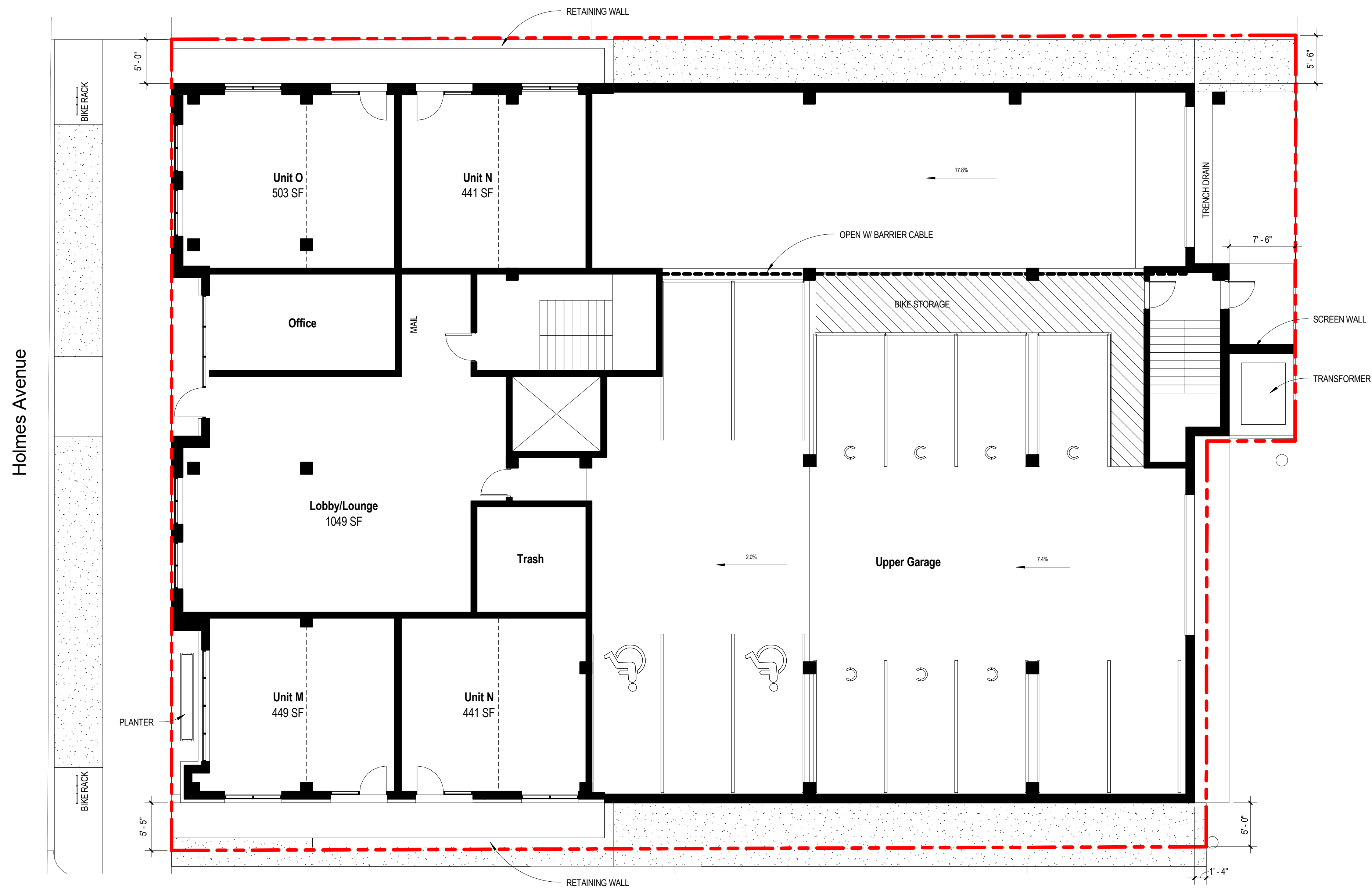
Plan - First Floor 1/8" = 1'-0"
