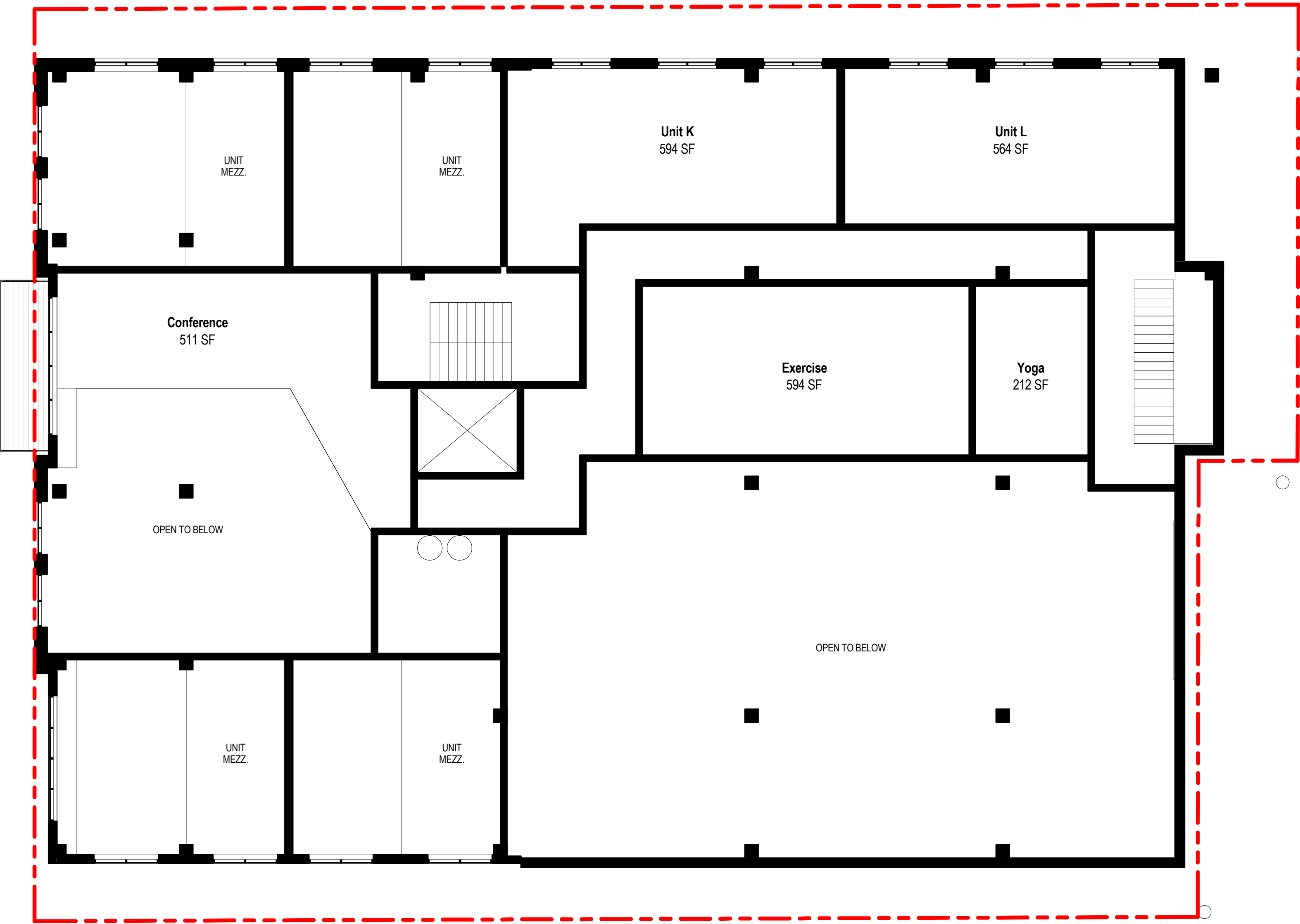
Plan - First Floor Mezzanine 1/8" = 1'-0"
