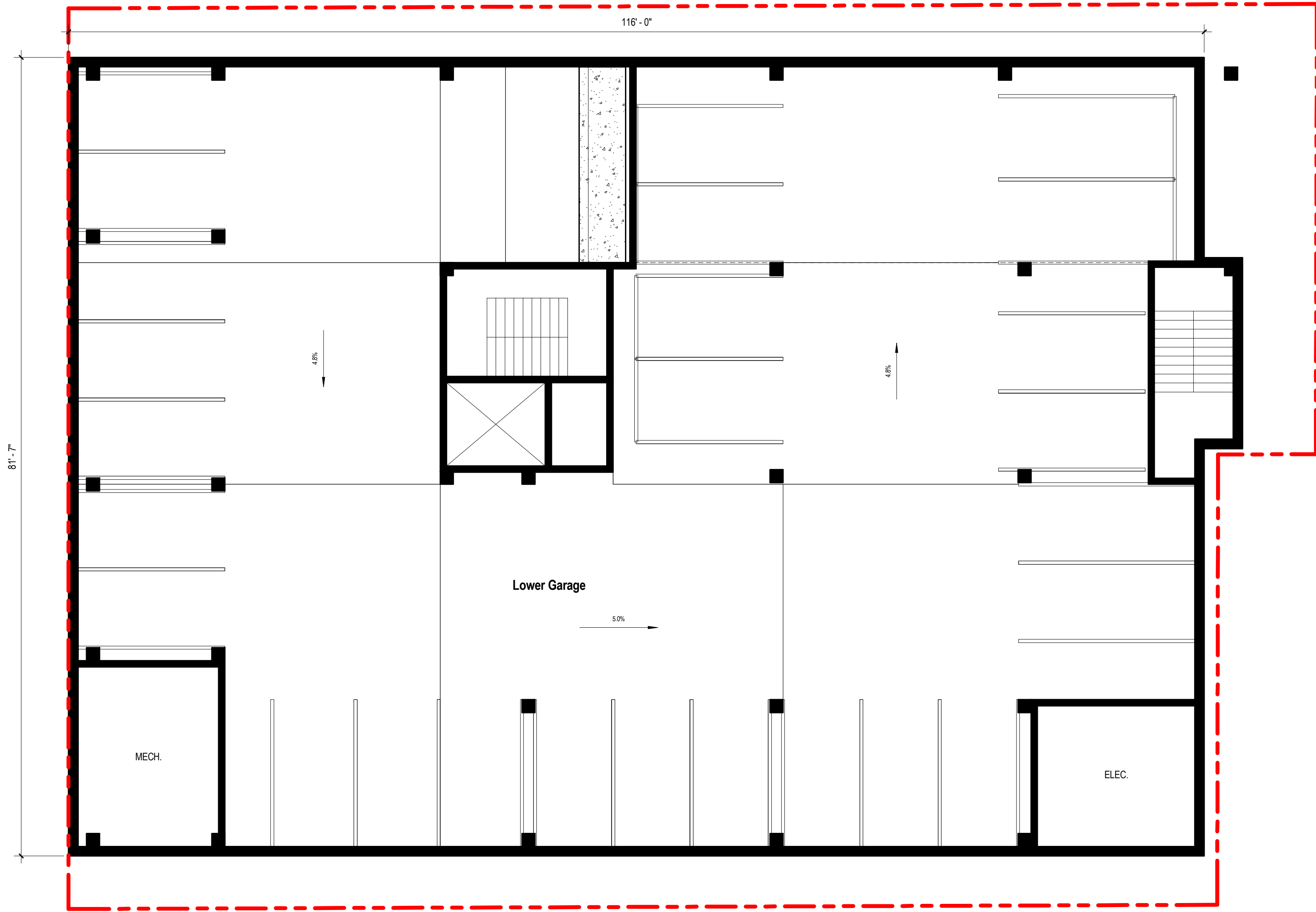
Plan - Basement Floor 1/8" = 1'-0"
