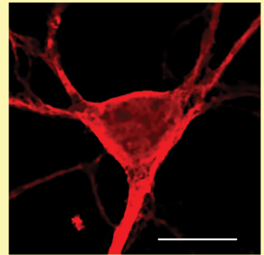
NDCBE
